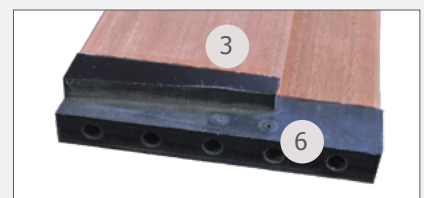
Images show the bottom corner of door (1), sill (5) and jamb leg (3) (6).
