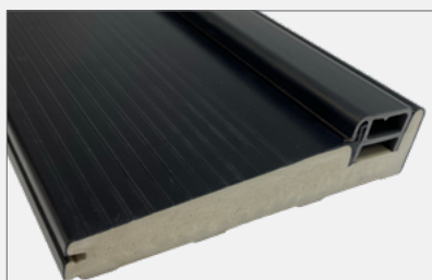
STANDARD SILL with Composite substrate that will not warp or rot. Available in both Bronze (shown here) and Mill finishes.
